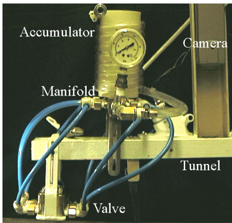
Fig. 1 Robotic spraying system.
